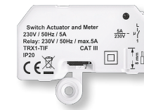
DITECH Smart Home Unterputz-Schalt-Mess-Aktor neutral Art.-Nr. DT5648
